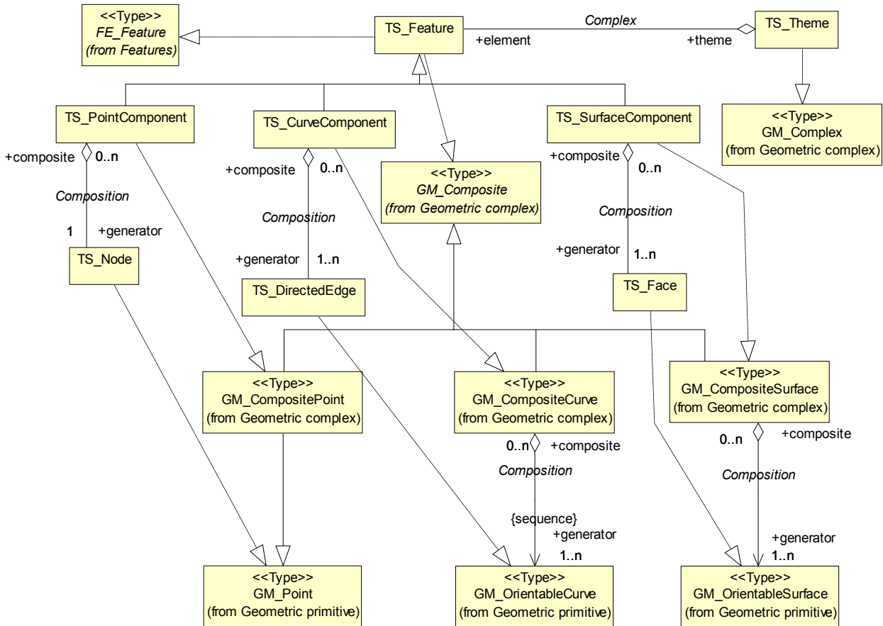
Figure D.3 — Feature components in simple topology
