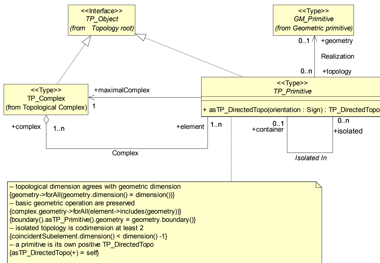
Figure 38 — TP_Primitive
