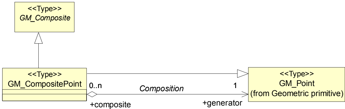
Figure 27 — GM_CompositePoint
