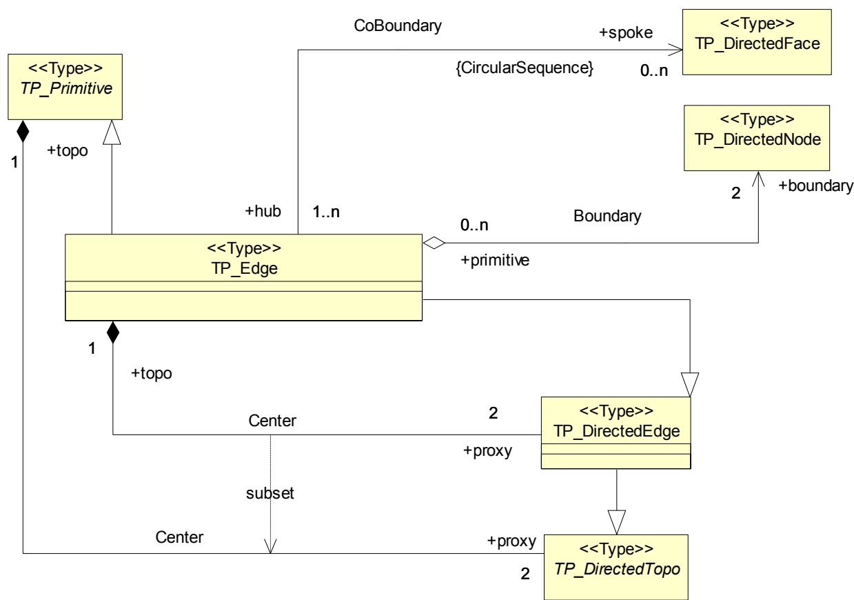
Figure 42 — TP_Edge
