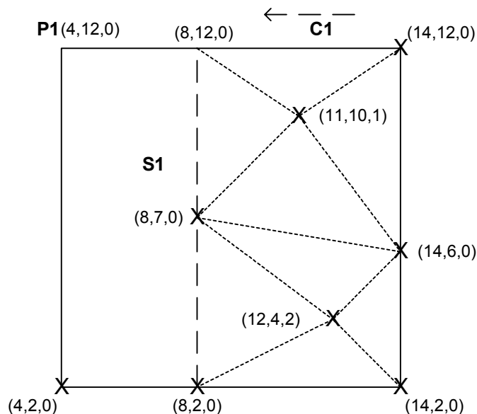
Figure C.4 — Surface example
