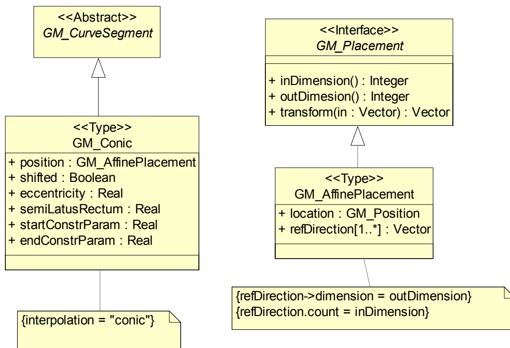
Figure 18 — Conics and placements
