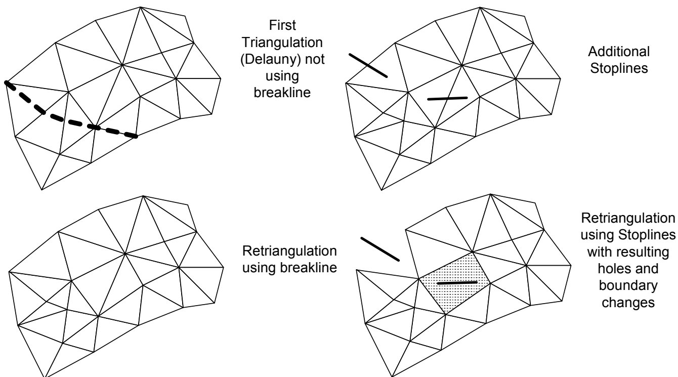
Figure 22 — TIN construction
