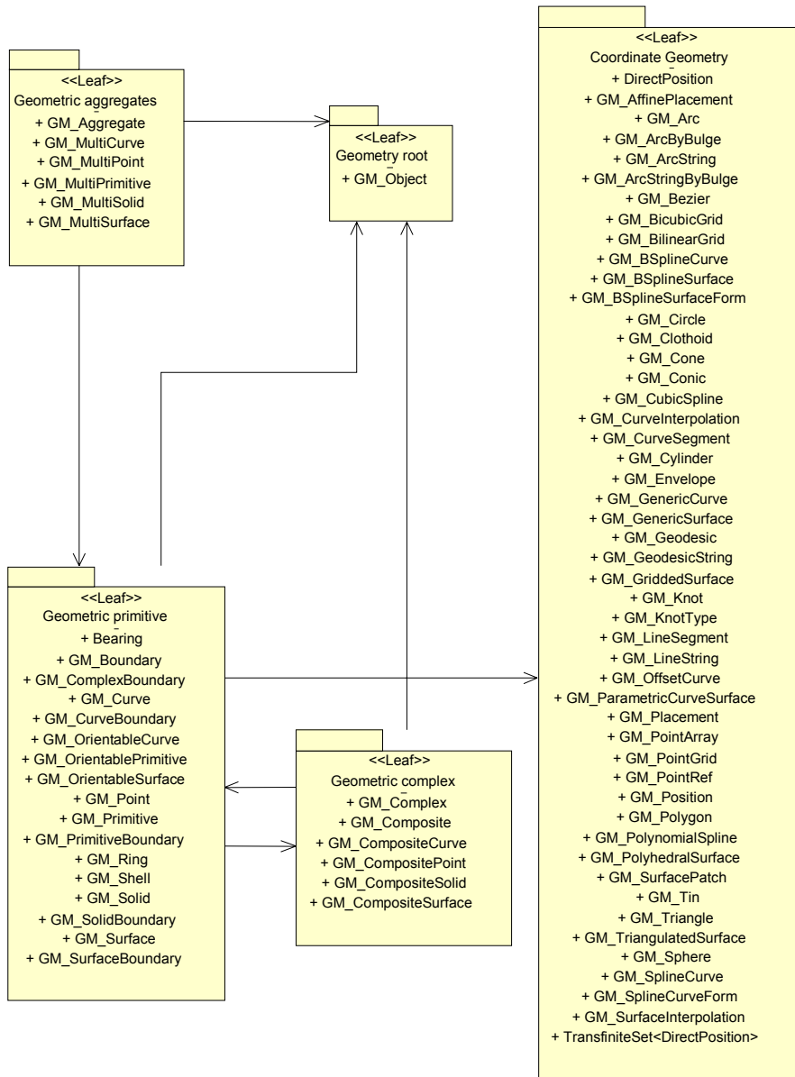
Figure 4 — Geometry package: Class content and internal dependencies
